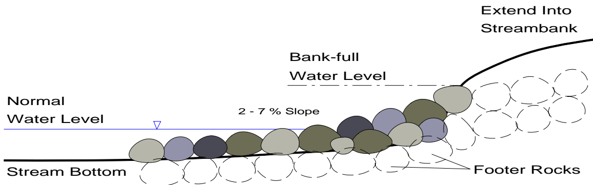
Section View
