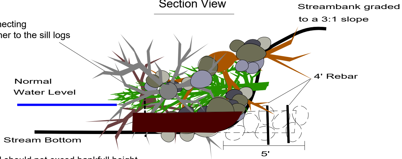
Section View
