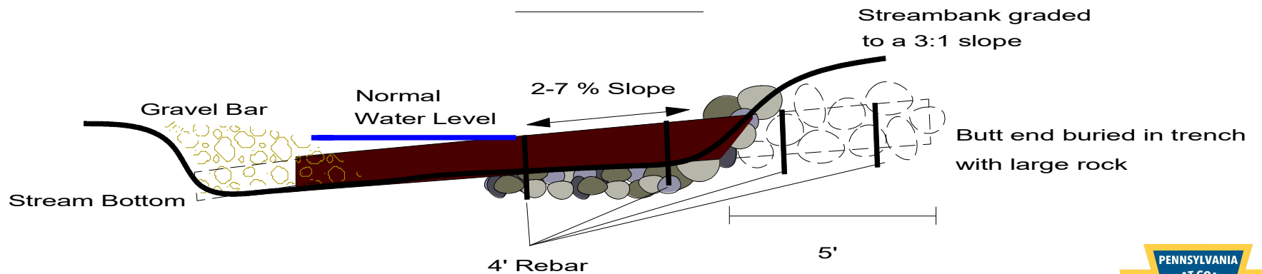
4' Rebar Pin
