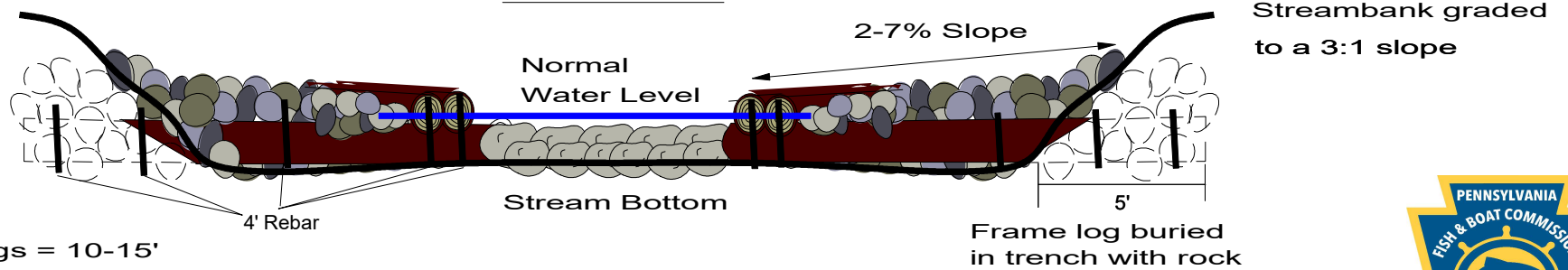
Section View
